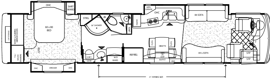
Model Shown: EXDP 4501
